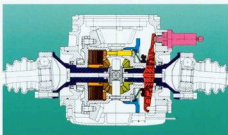
First proven on the awesome Porsche 959, the electronically variable limited slip differential automatically varies the locking action to provide higher stability and improved traction under all conditions.
